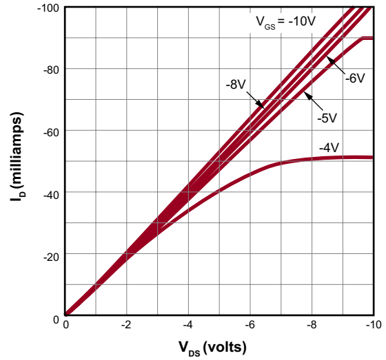
Saturation Characteristics
